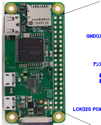
Raspberry Pi Zero WH
